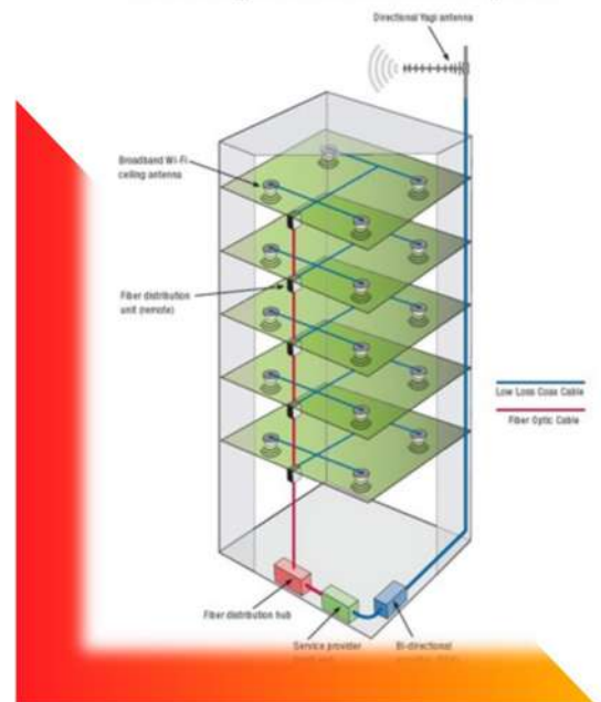
In-Building Distributed Antenna System
